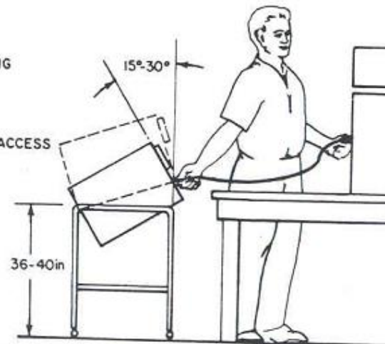
PORTABLE TEST STAND (ADJUSTABLE ANGLE FOR TEST EQUIPMENT)
