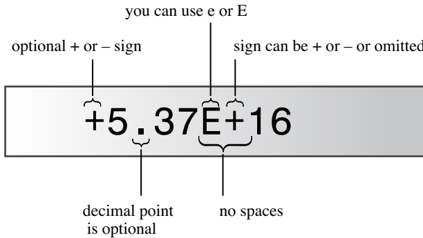
Figure 3.3 E notation.
