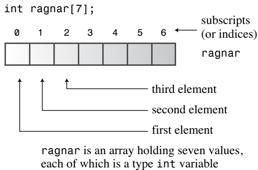
Figure 4.1 Creating an array.
