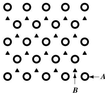
FIGURE H.2 Sequence of close-packed planes \{0001\} in HCP lattice.
