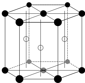
FIGURE H.1 Unit cell of HCP lattice.
