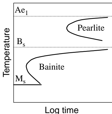
FIGURE T.3 TTT diagram for eutectoid alloy steel (scheme).
