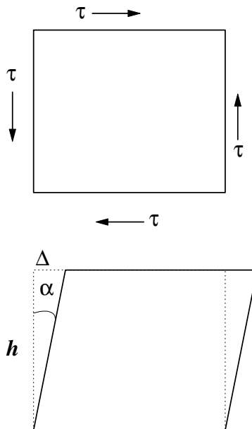
FIGURE S.1 Shear and shear strain. Above: before shear. Shear stresses \tau are applied not only to horizontal faces of the parallelepiped, but also to its side faces; the latter is necessary to prevent rotation of the parallelepiped. Below: after shear. See text.
