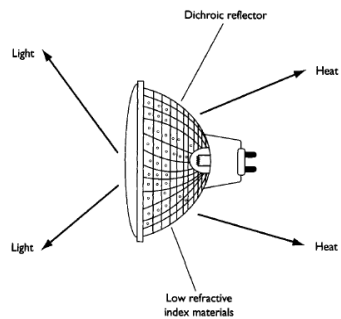
Figure 7.7 Dichroic reflector lamp.
