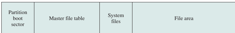
Figure 12.21 NTFS Volume Layout
