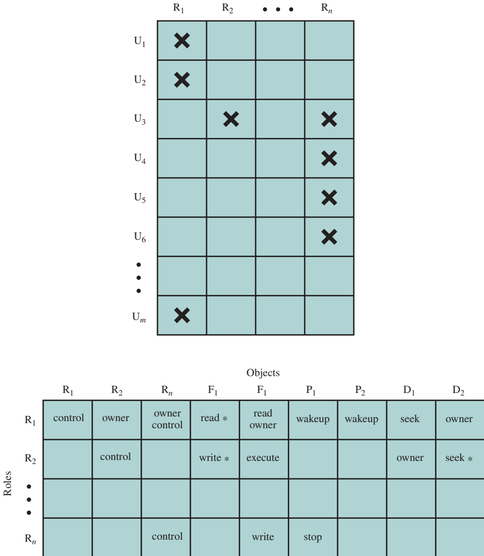
Figure 15.7 Access Control Matrix Representation of RBAC
