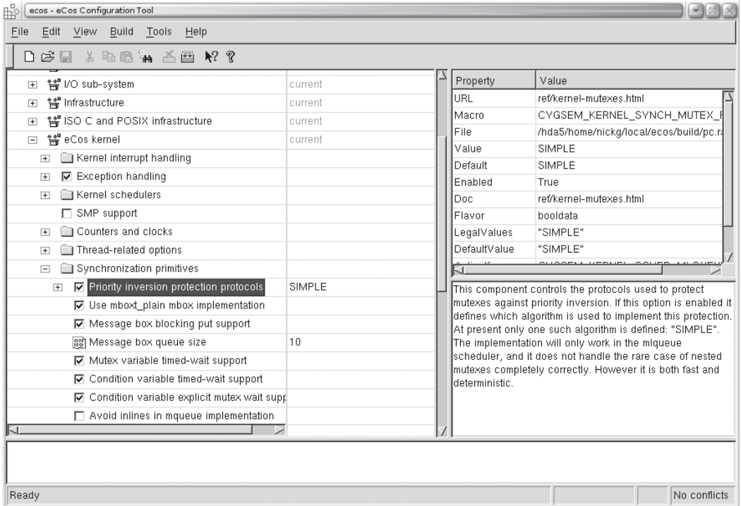
Figure 13.3 eCos Configuration Tool—Kernel Details
