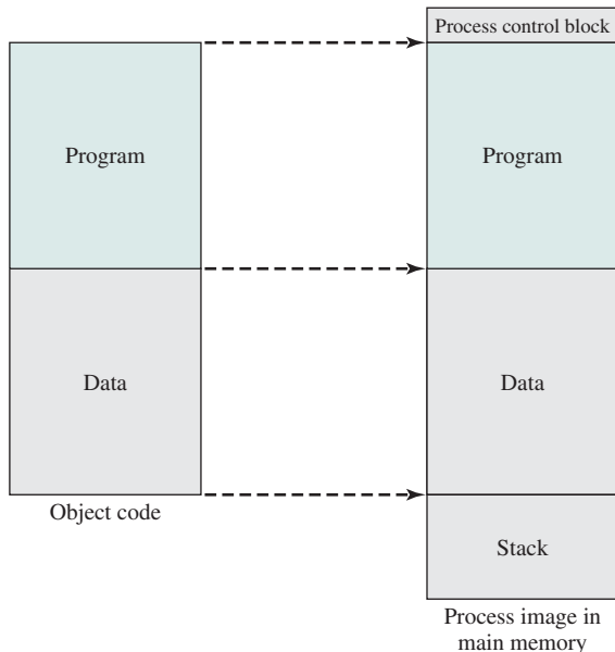
Figure 7.15 The Loading Function
