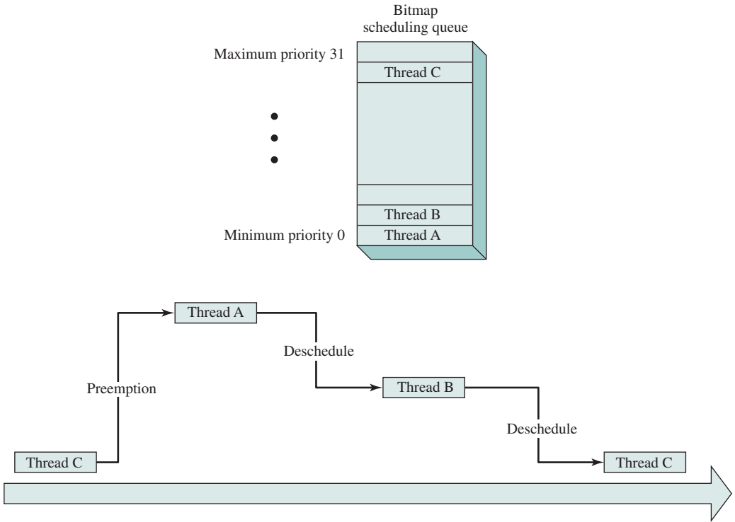
(a) Bitmap scheduler thread operation
