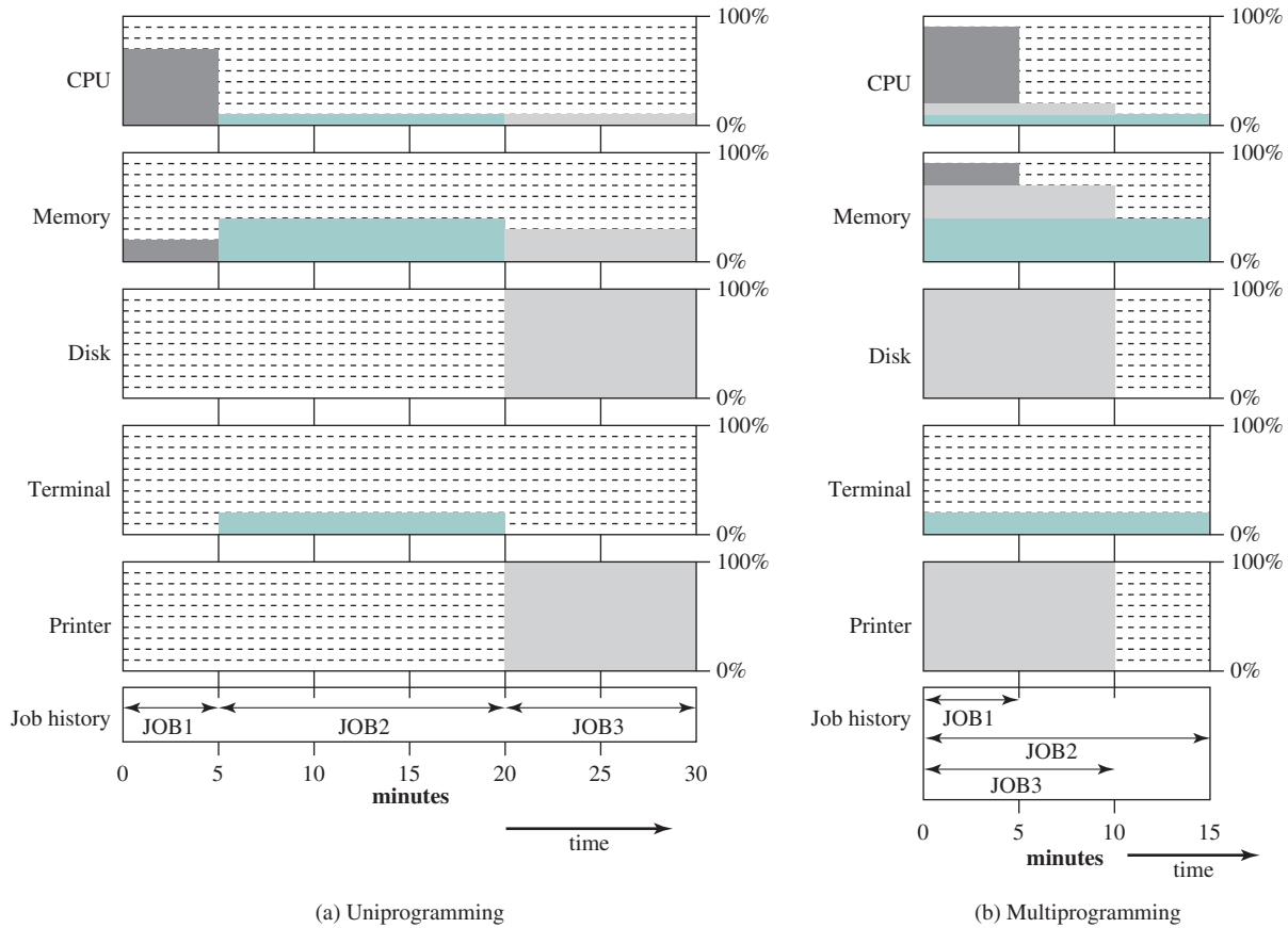
Figure 2.6 Utilization Histograms
