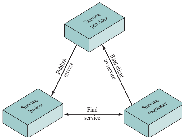
Figure 16.10 SOA Model
