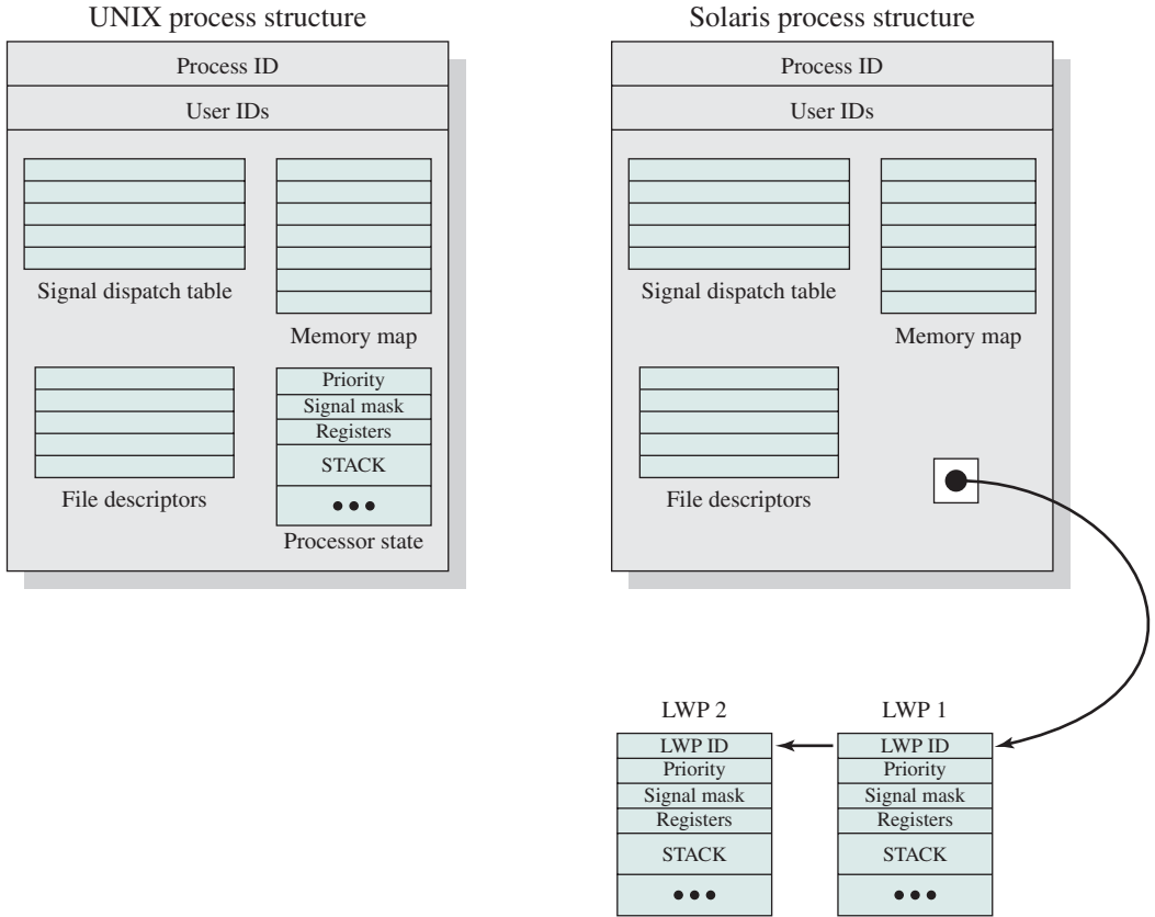
Figure 4.14 Process Structure in Traditional UNIX and Solaris [LEWI96]
