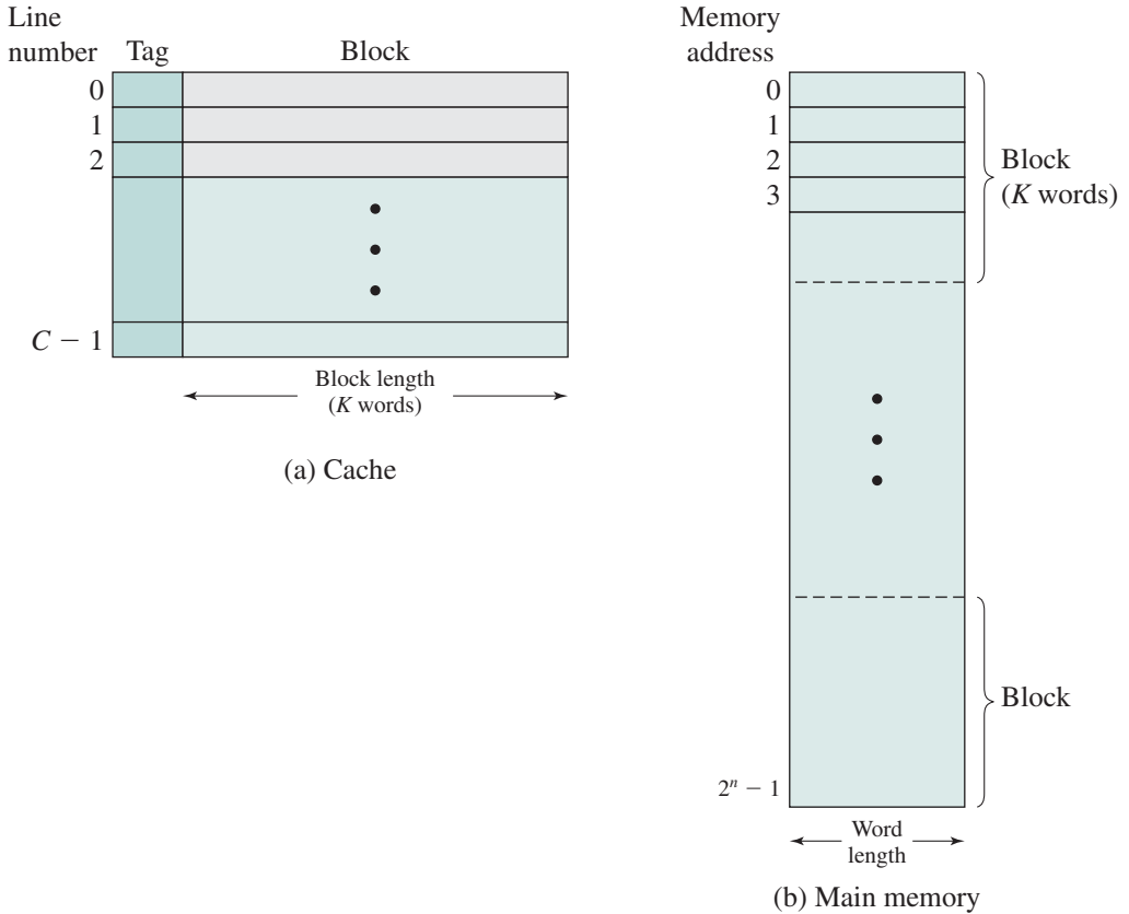
Figure 1.17 Cache/Main-Memory Structure
