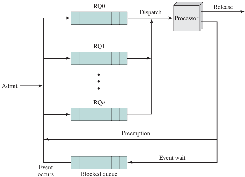
Figure 9.4 Priority Queuing
