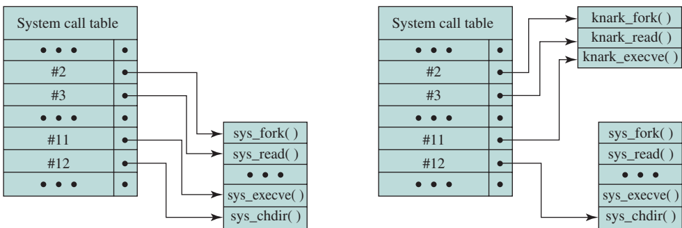
(a) Normal kernel memory layout
