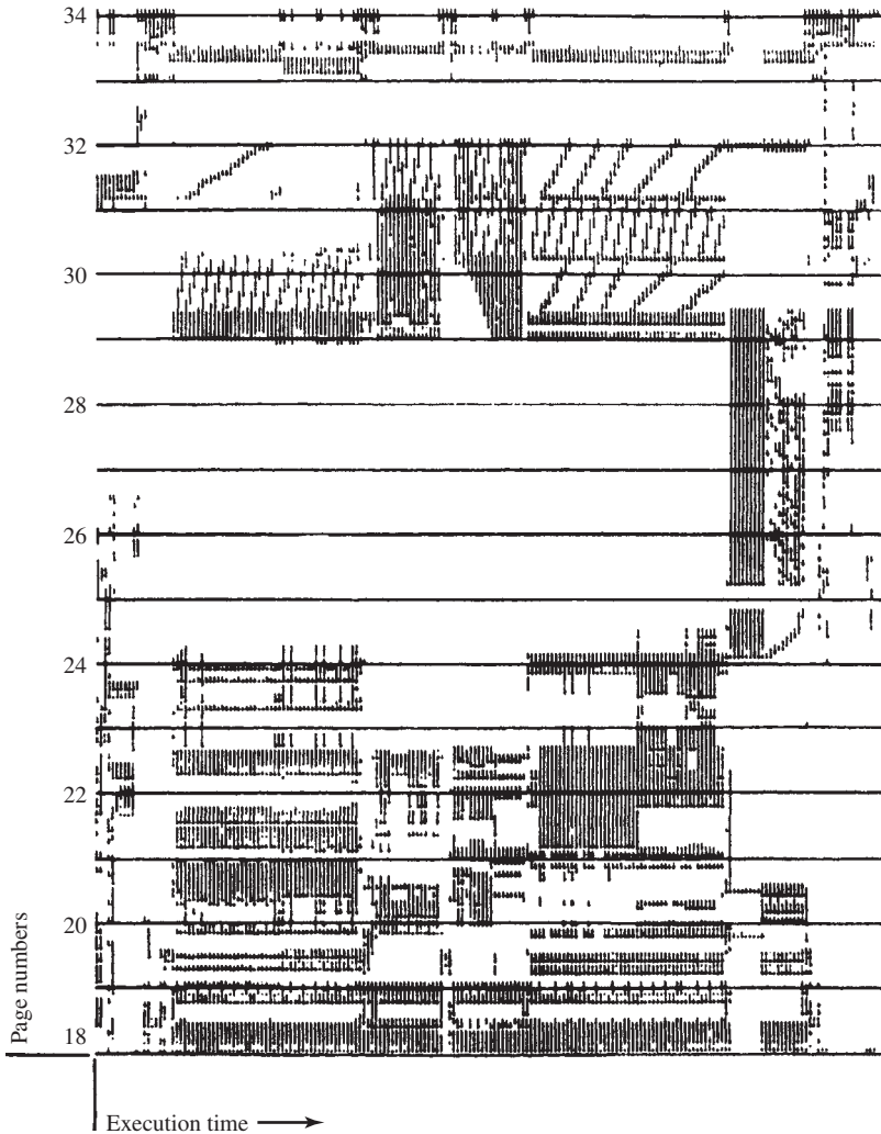
Figure 8.1 Paging Behavior
