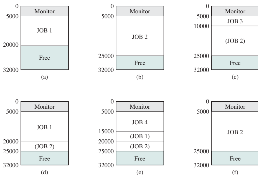
Figure 2.7 CTSS Operation
