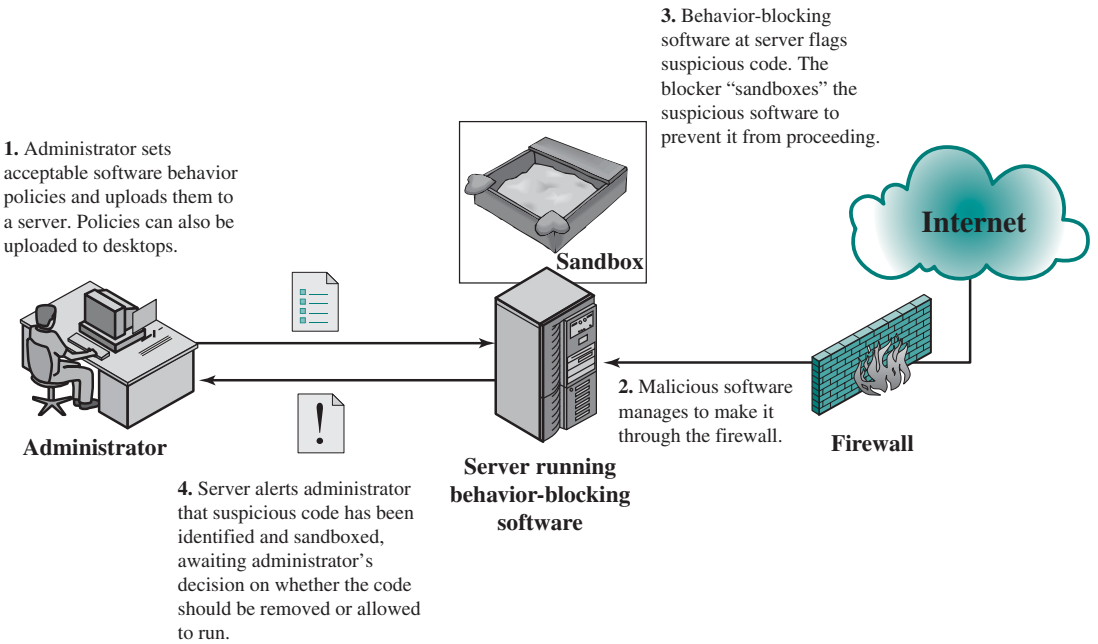
Figure 15.10 Behavior-Blocking Software Operation
