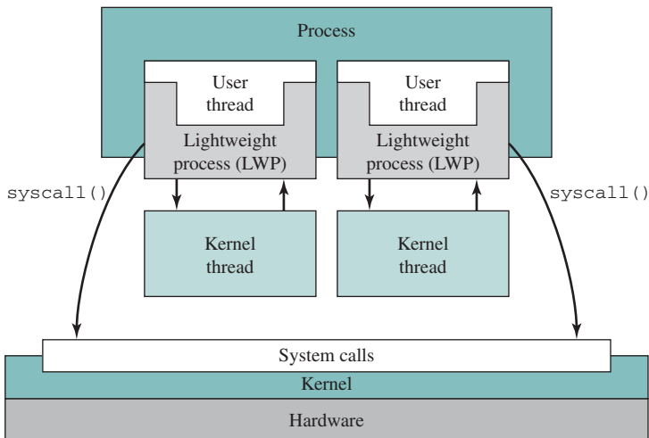
Figure 4.13 Processes and Threads in Solaris [MCDO07]
