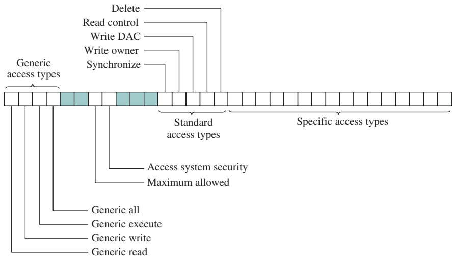
Figure 15.12 Access Mask
