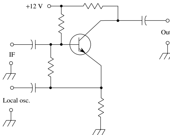
product detector
