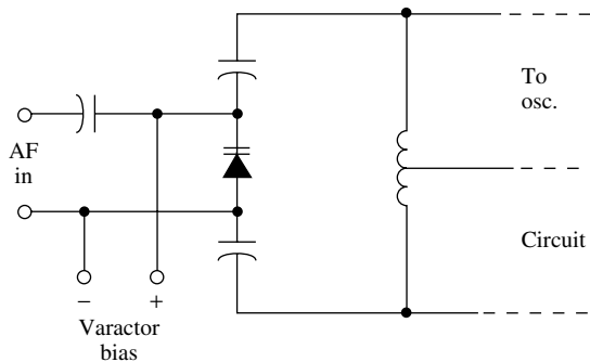
reactance modulator
