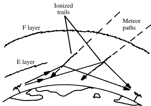
meteor-trail reflections
