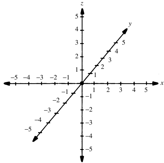
Cartesian three-space
