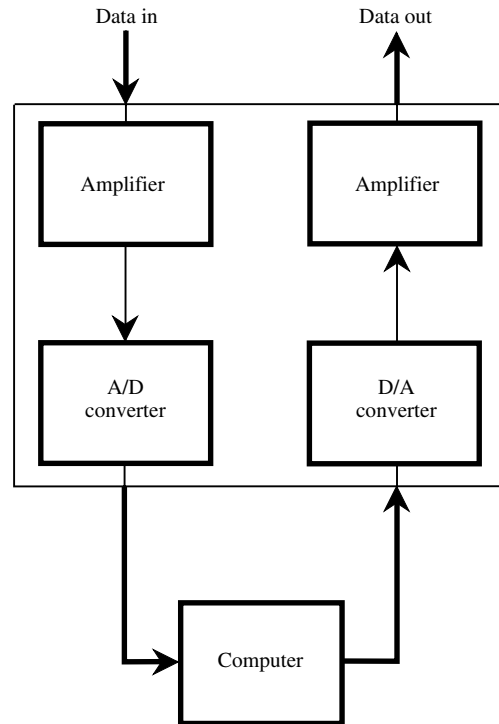
modulator-demodulator
