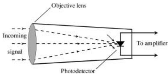
optical antenna
