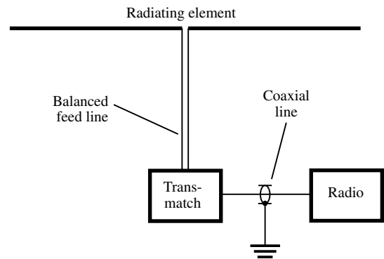
multiband antenna
