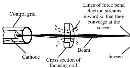
electromagnetic focusing
