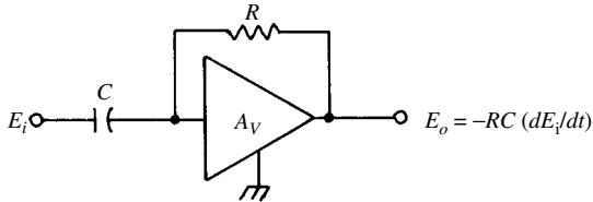
differentiator, 2
