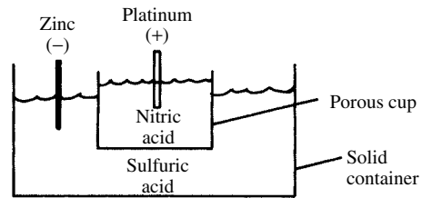
Grove cell
