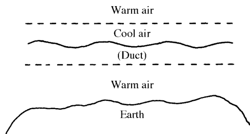
atmospheric duct
