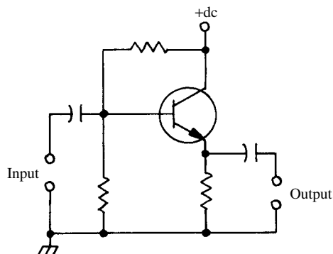
emitter follower
