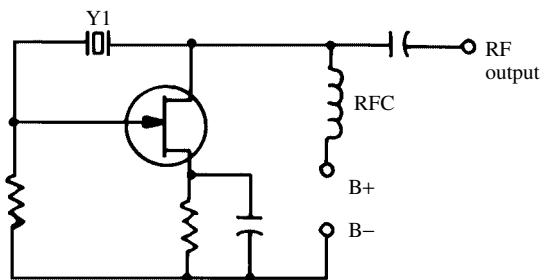
Pierce oscillator
