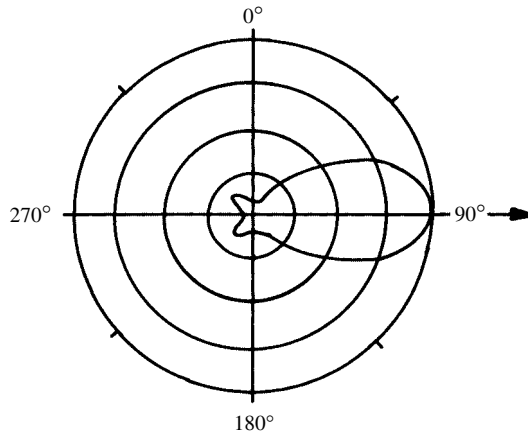
unidirectional pattern
