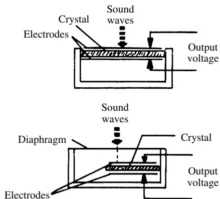
crystal microphones
