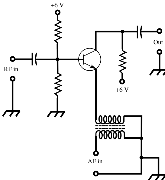
modulated amplifier
