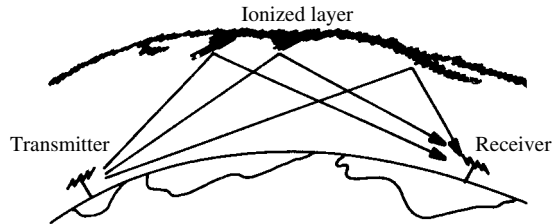
multipath reception
