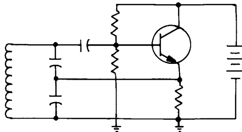
Colpitts oscillator
