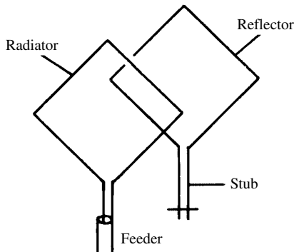
quad antenna
