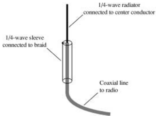
coaxial antenna
