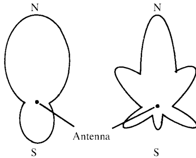
antenna patterns
