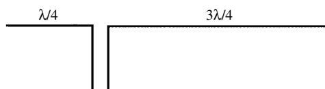
off-center feed
