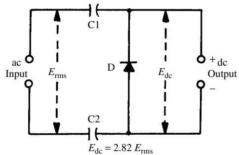
Villard circuit, 1
