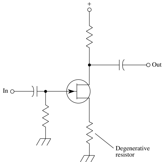
degenerative resistor
