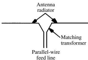
delta-matching transformer
