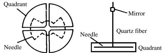
quadrant electrometer
