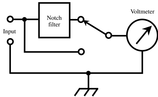
distortion meter
