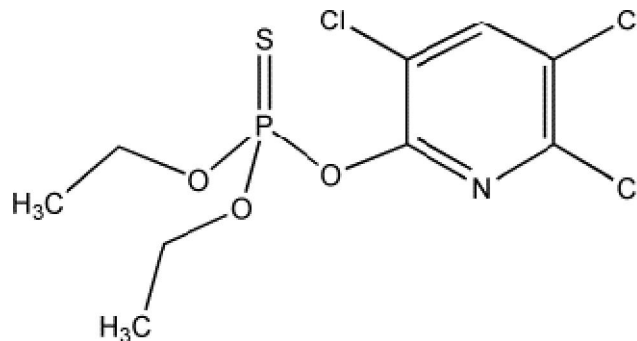
Chlorpyrifos (Lorsban)
