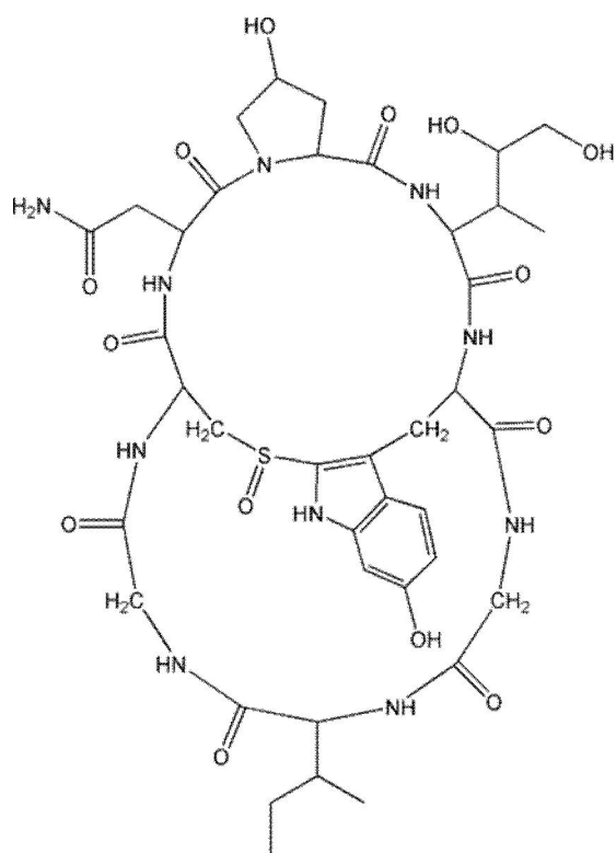
Alpha-amanitin(Amatoxins)
