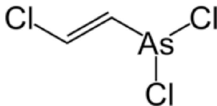
Lewisite
