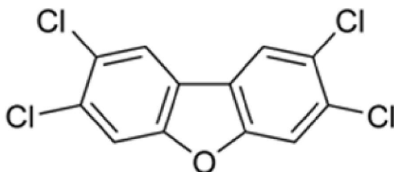
2,3,7,8-tetrachlorodibenzofuran (TCDF)
