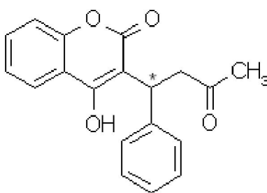
Warfarin
