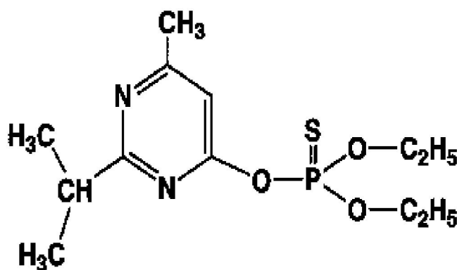
Diazinon
