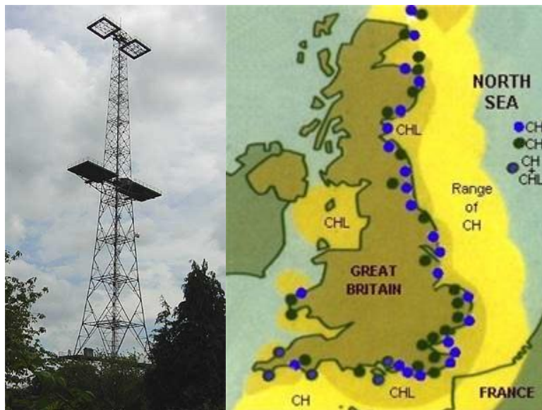
شكل ٢-٢ chain home and its coverage [7] [8]
