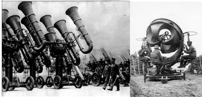
شكل ٣-٢ acoustic location [6]
